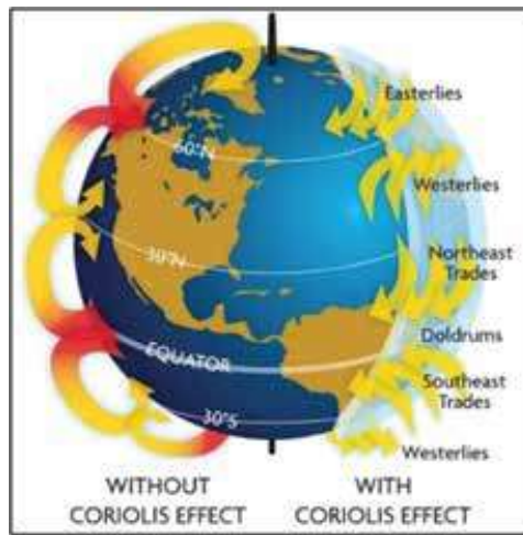
Figure 2: The Coriolis Effect. 2
