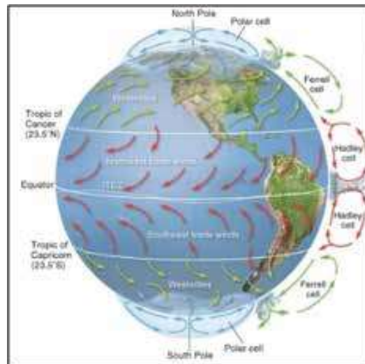
Figure 1: Global atmospheric circulation model. 1
