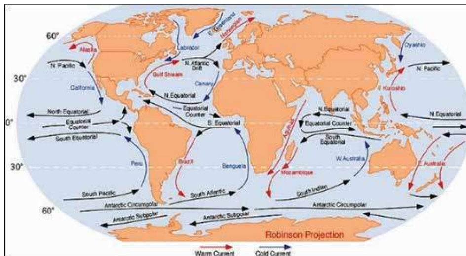
Figure 4: The general movement of the currents in the northern hemisphere is clockwise and in the southern hemisphere, anticlockwise. 5
